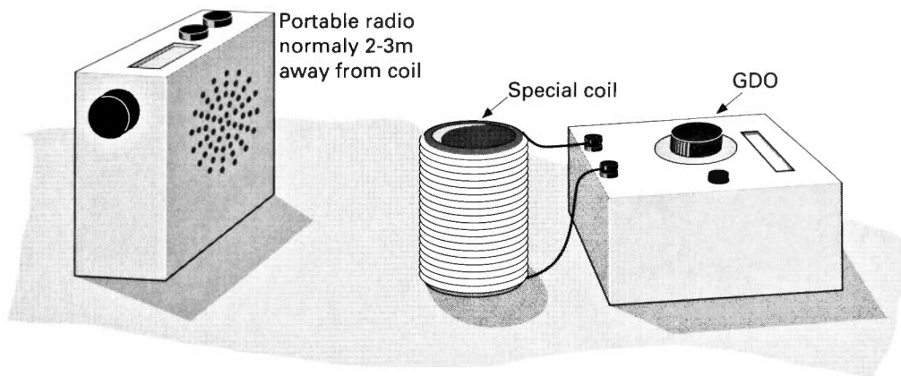
Fig. 4: Showing the method used to calibrate the dial for any new coil. The portable radio can be almost any good receiver, with suitable frequency coverage, of known accuracy.
