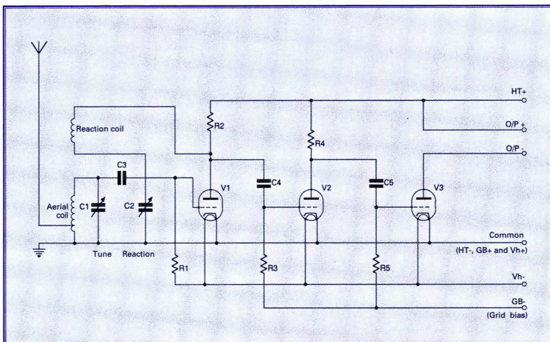
Fig. 1: Wilfred Harms built this circuit over 60 years ago. Although he cannot remember individual component values, or exactly which magazine published the project, he was pleased that it worked well. In the text Wilfred explains how he had to make resistors from strips of newsprint and metal polish, and capacitors from metal foil. The receiver met its end when his mother wanted the kitchen table back!
