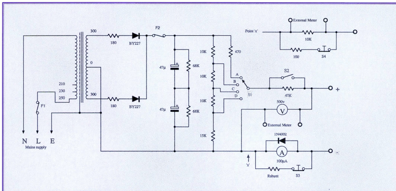
Fig. 4: Simple electrolytic reformer and tester circuit. Electrolytic capacitors have very thin chemical dielectrics that can deteriorate and become leaky after a period of non-use. Applying the full rated voltage to a capacitor in this state can result in an explosion. Before use, all medium to high voltage electrolytics should be reformed by applying the full working voltage through a high value resistor. Initially the high leakage current will cause a substantial voltage drop across the resistor. This will gradually reduce as the capacitor recovers. After some hours, the leakage current will gradually stabilise to a low value. The voltage across the capacitor will have correspondingly increased. However, if the capacitor is still drawing a high leakage current after 24 hours, it should be discarded.
