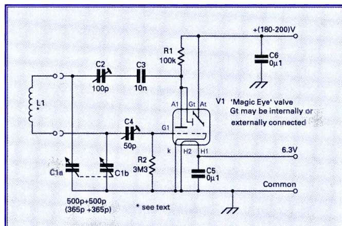
Fig. 1: Circuit of the magic eye valved grid-dip oscillator. See Table 1 for the valve pin connections, and alternative valves.
