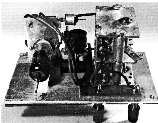
Fig. 3: The inside of the g.d.o. showing the layout of the major components and the magic eye mounted behind the slot cut in the front panel.
