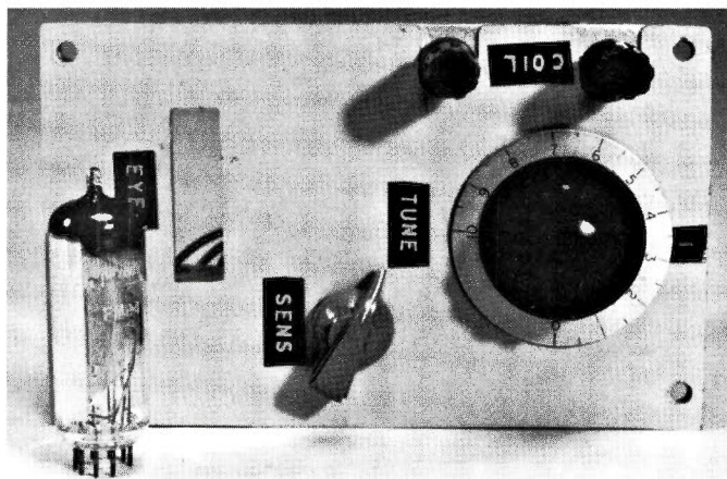
The practical g.d.o. circuit using a magic eye tuning indicator in place of a moving coil meter.
