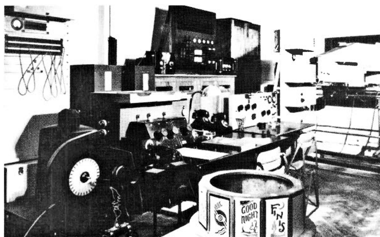
Fig. 4: The BBC television control room at 16 Portland Place in London in 1935. Caption machine in foreground, with disc scanner on the left, with twin monitor receivers above. The mirror-drum scanner (the camera) is pointing into the studio.
