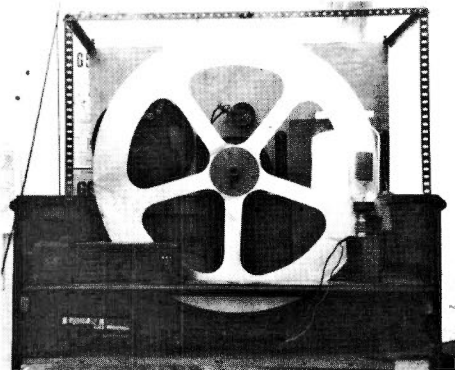
Fig. 3: Home-constructed 30-line mechanical scanning television, built by Ray Herbert G2KU as a schoolboy in 1933. The flat plane neon tube for picture illumination is shown on the right.
