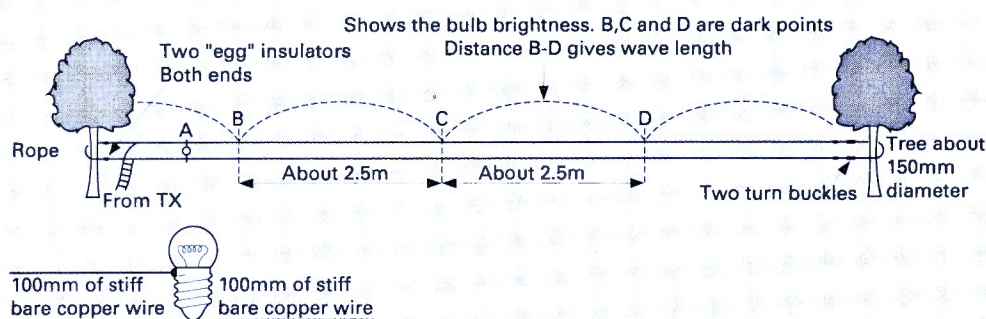
Fig. 8: Diagram illustrating the Lecher line technique G6XM used to find the correct wavelengths for the old 5 metre band. Also shown is the block diagram of G6XM's 5 metre transmitter, clearly illustrating the useful harmonic relationships of the pre-1939 amateur radio bands.
